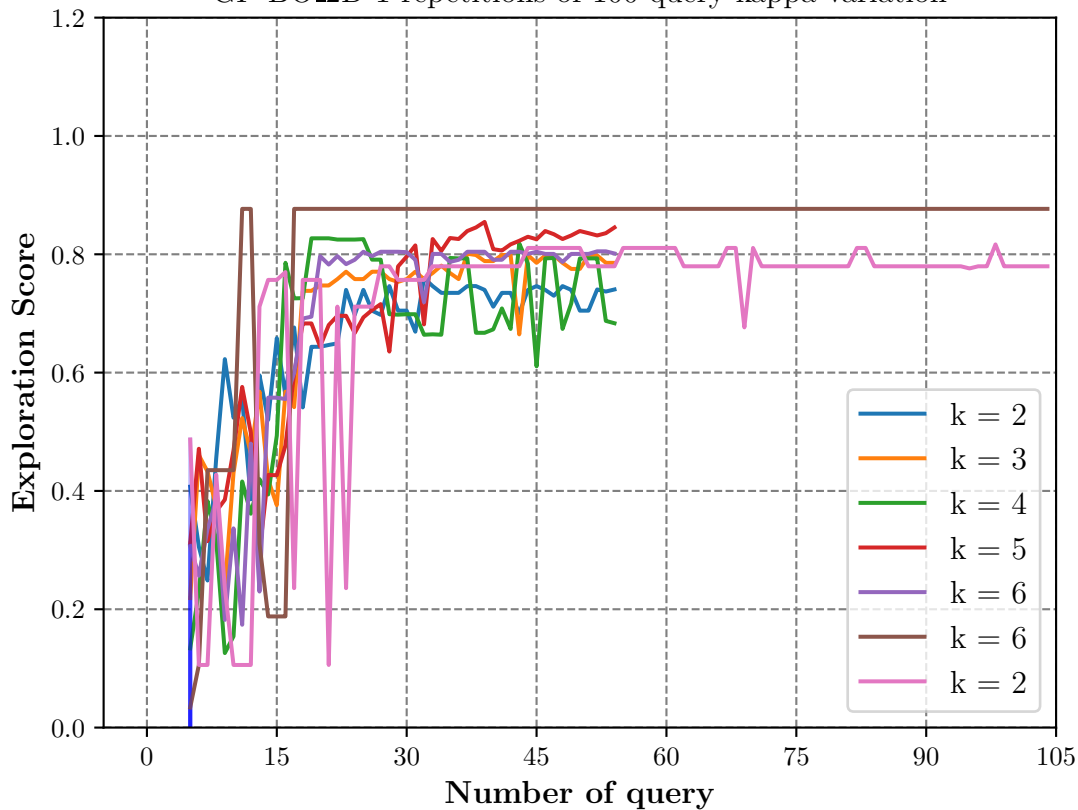
GP-BO_2D 1 repetitions of 100 query kappa variation
